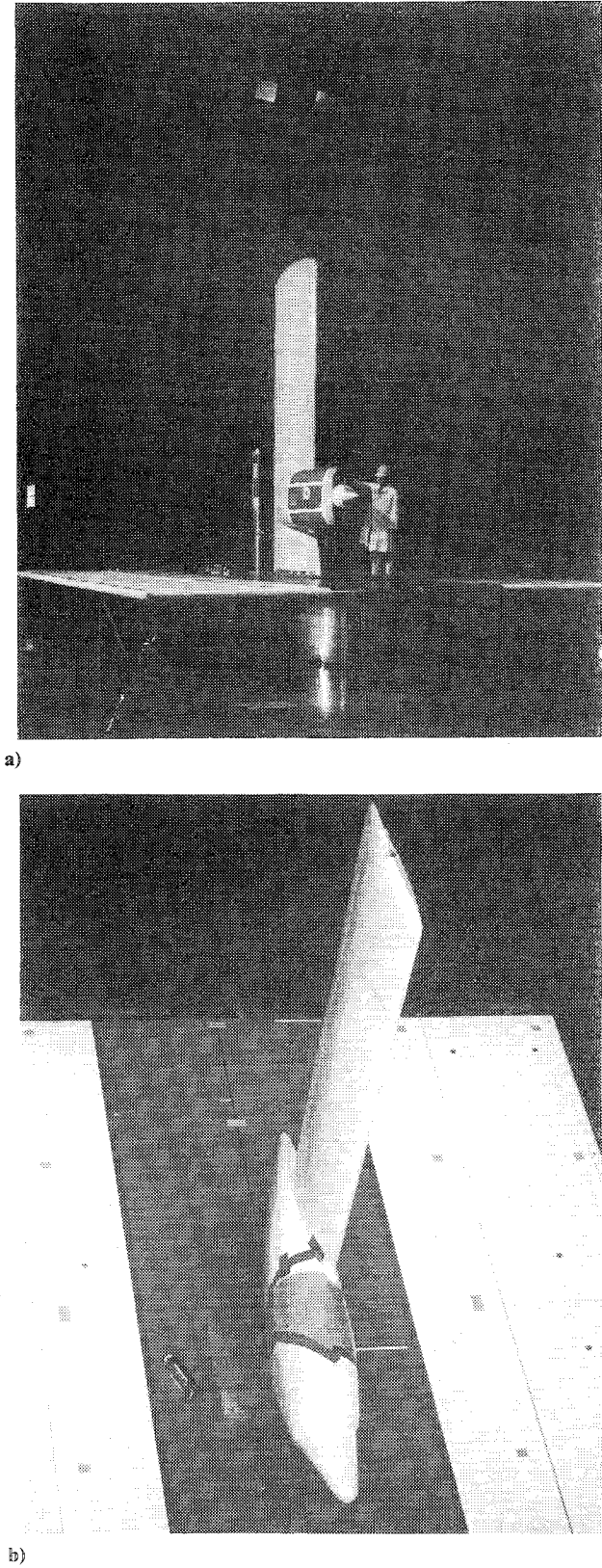
Fig. 3 Wing installed in Ames 40 by 80 ft Wind Tunnel: a) test configuration, b) reference configuration.
