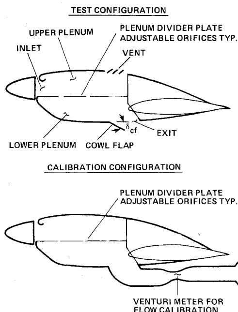
Fig. 4 Nacelle arrangement illustrating venturi meter for orifice calibration.
