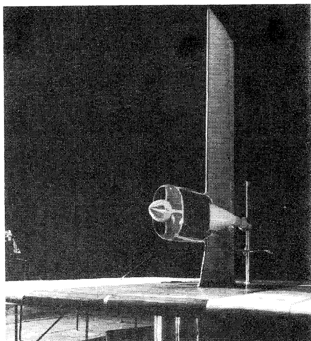
Fig. 5 Venturi meter and aft momentum rake.
