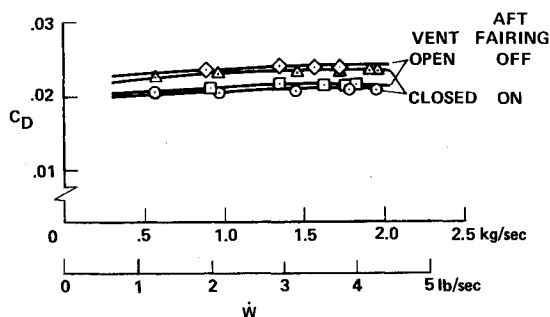
Fig. 11 Effect on drag caused by opening and closing upper plenum vent (scale data): \alpha = 2.3 deg, V_\infty = 156 knots.
