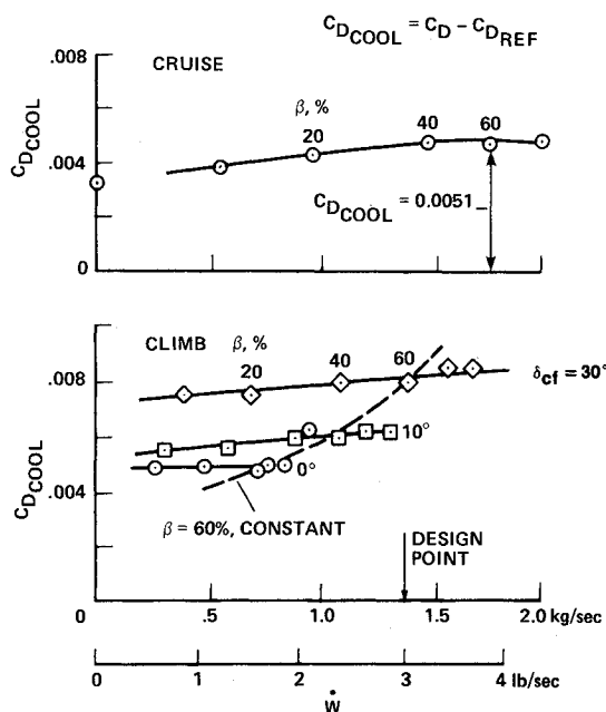
Fig. 10 Cooling drag (scale data) ( C_{D_{COOL}} = C_D - C_{D_{REF}} ) as function of cooling flow rate for both cruise and climb conditions, aft fairing on: cruise, \alpha = 2.3 deg, V_\infty = 156 knots; climb, \alpha = 8 deg, V_\infty = 94 knots.
