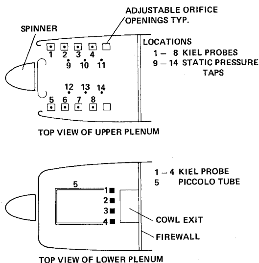
Fig. 6 Nacelle internal pressure instrumentation.
