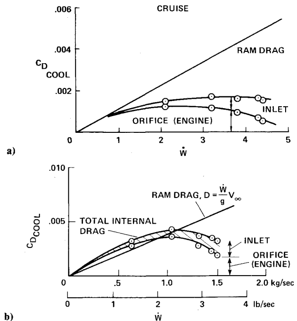
Fig. 14 Internal nacelle cooling drag as determined by total pressure and flow rate in upper and lower plenum, aft fairing on: a) cruise, \alpha = 2.3 deg, V_\infty = 156 knots, \delta_{cf} = 0 deg; b) climb, \alpha = 8 deg, V_\infty = 94 knots, \delta_{cf} = 30 deg.
