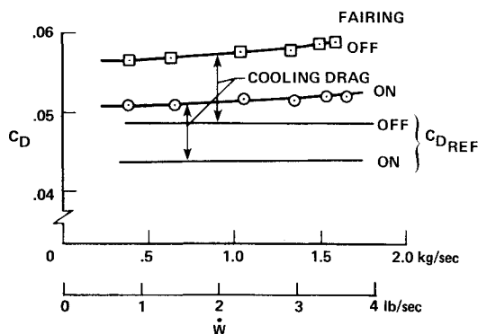
Fig. 7 Effect of aft fairing on drag (scale data) for both test and reference configurations: climb: \alpha = 8 deg, V_\infty = 94 knots, \delta_{cf} = 30 deg.
