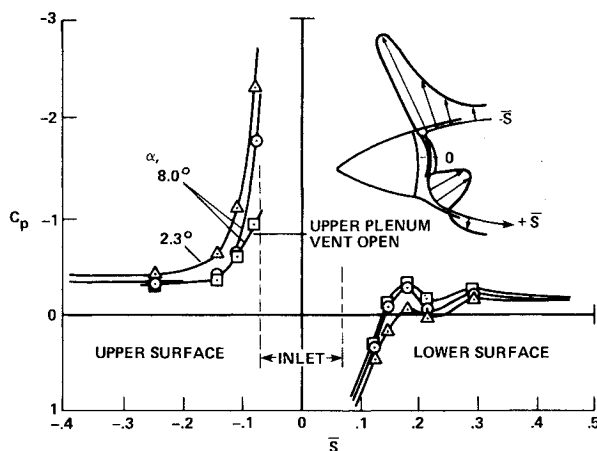
Fig. 9 Streamwise contours of surface pressure along curve passing vertically through cooling inlet: \dot{W} = 1.2 kg/s (2.7 lb/s), V_\infty = 156 knots ( \alpha = 2.3 deg), V_\infty = 94 knots ( \alpha = 8 deg), aft fairing off.
