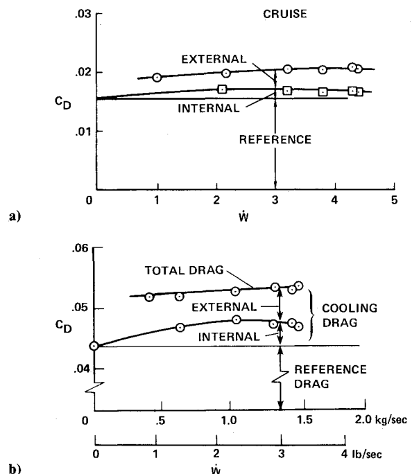
Fig. 15 Summary of drag coefficient breakdown, aft fairing on: a) cruise, \alpha = 2.3 deg, V_\infty = 156 knots, \delta_{cf} = 0 deg; b) climb, \alpha = 8 deg, V_\infty = 156 knots, \delta_{cf} = 30 deg.
