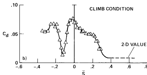
Fig. 8 Section drag coefficient as function of span as determined by integration of static and total pressures on wake momentum rake, aft fairing off: a) cruise, \alpha = 2.3 deg, V_\infty = 156 knots, \delta_{cf} = 0 deg; b) climb, \alpha = 8 deg, V_\infty = 94 knots, \delta_{cf} = 30 deg.
