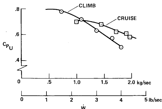
Fig. 13 Upper plenum total pressure, aft fairing on: climb, \alpha = 8 deg, V_\infty = 94 knots, \delta_{cf} = 30 deg; cruise, \alpha = 2.3 deg, V_\infty = 156 knots, \delta_{cf} = 0 deg.
